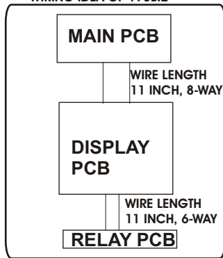
WIRING IDEA OF 193BI2
